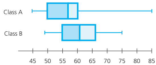
Figure 10.9 Boxplots
