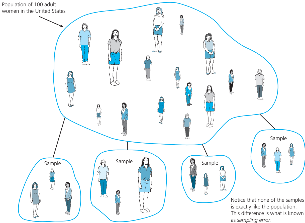
Figure 11.2 Sampling Error
