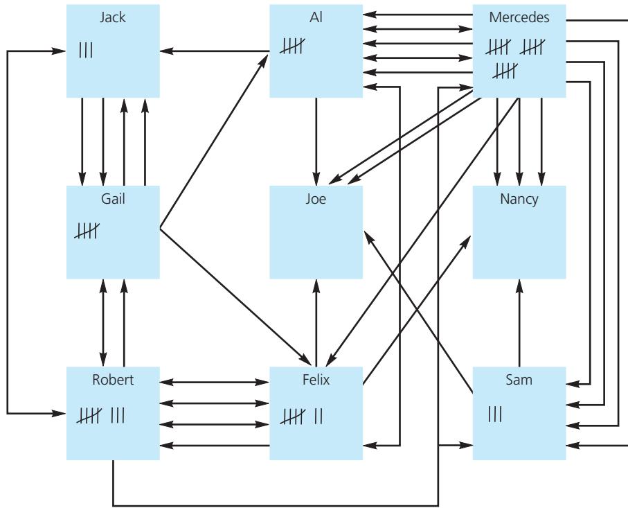
Figure 7.11 Participation Flowchart
