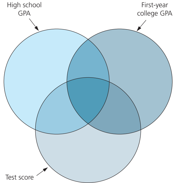
Figure 15.3 Multiple Correlation
