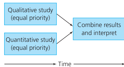
Figure 23.3 Triangulation Design
